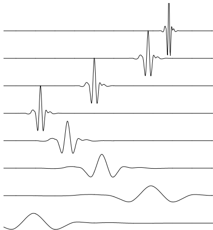
Figure 1: Localized Modes.
