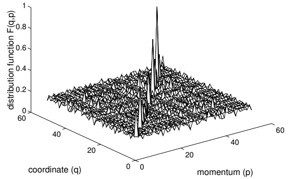
Figure 6: Goal: Localized Partition.
