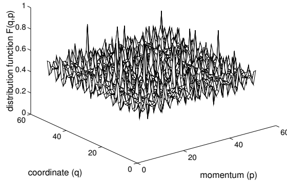
Figure 5: Trash: Chaotic Partition.
