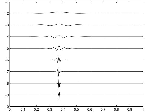
Figure 4: MRA for Kick.
