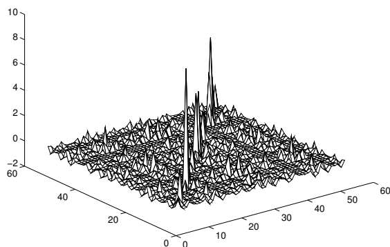
Figure 8: Fusion-like state: Wavelet Pattern.
