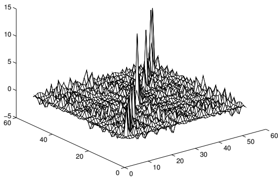
Figure 7: Fusion-like state: Confinement of Energy.
