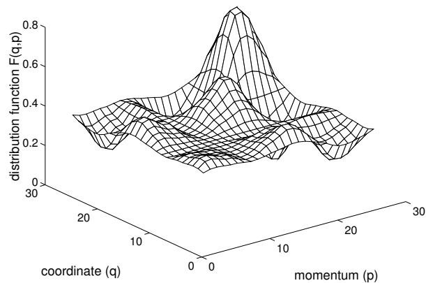
Figure 2: Two-dimensional Localized Mode Contribution to Distribution Function.
